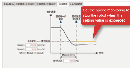
Speed monitoring setting
