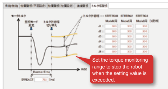
Torque monitoring setting
