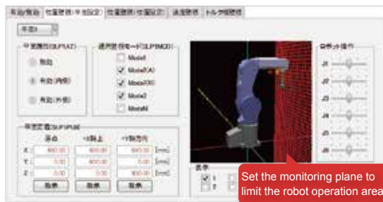
Position monitoring setting (plane setting)
