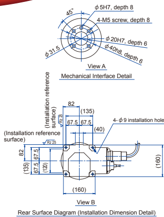
Rear Surface Diagram (Installation Dimension Detail)
